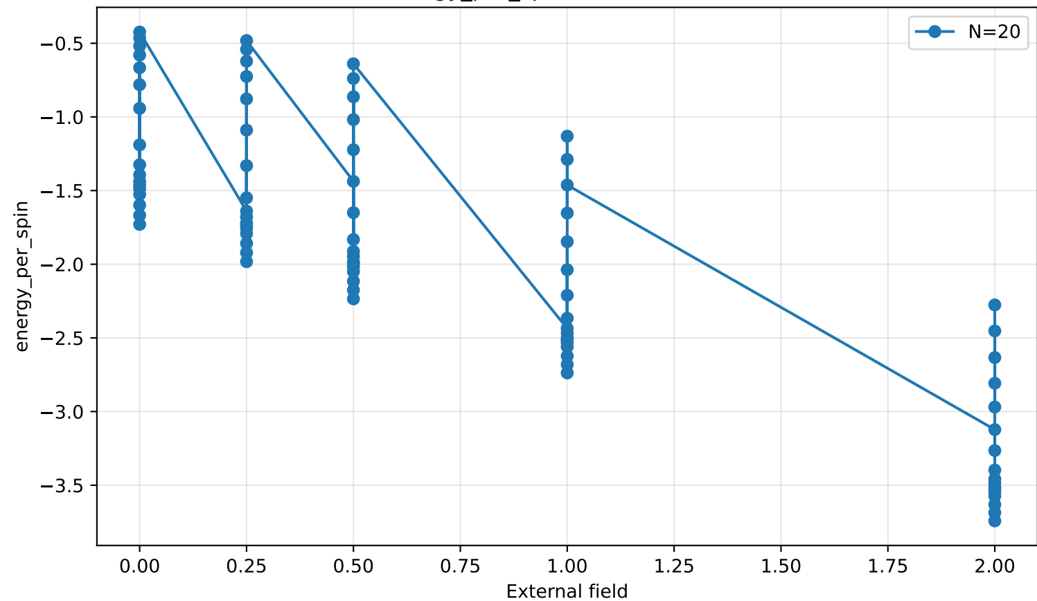
energy_per_spin vs external field
