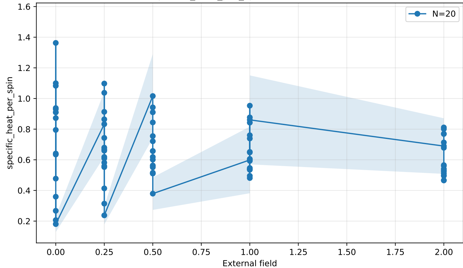
specific_heat_per_spin vs external field
