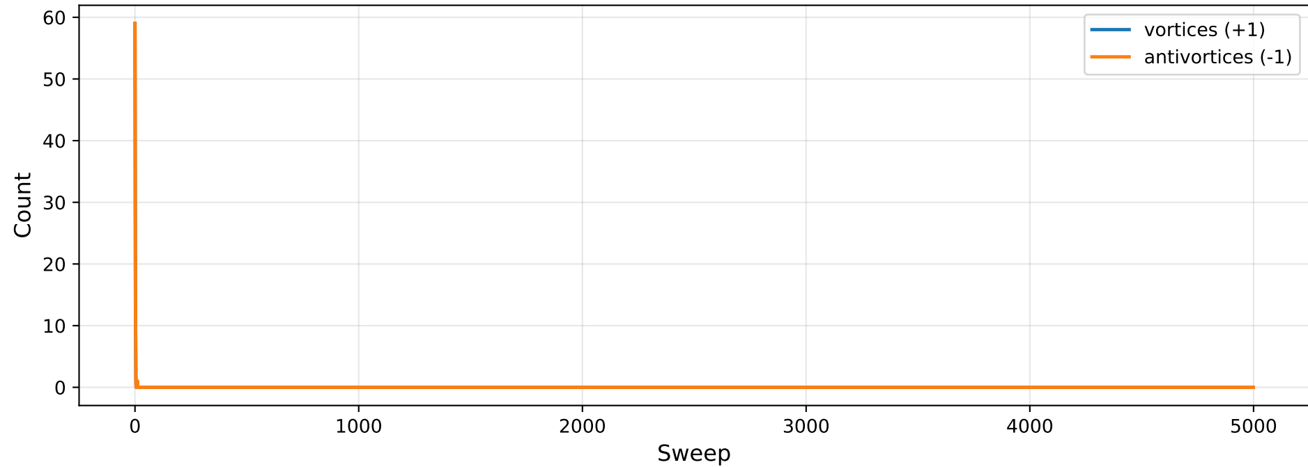
Vortices and antivortices vs sweep
