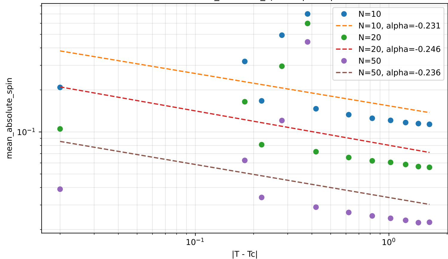
Power-law test: mean_absolute_spin vs |T - T_c| , T_c=0.88
