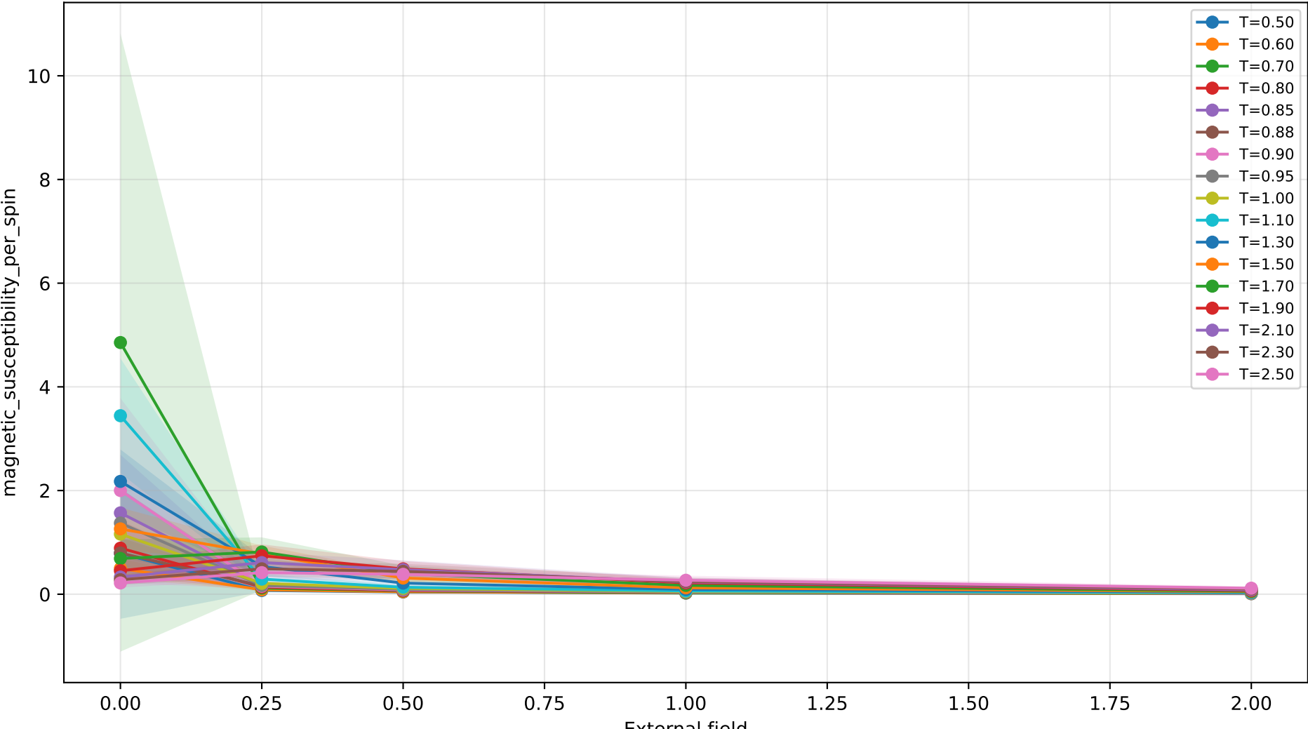
magnetic susceptibility per spin vs external field, N=20
