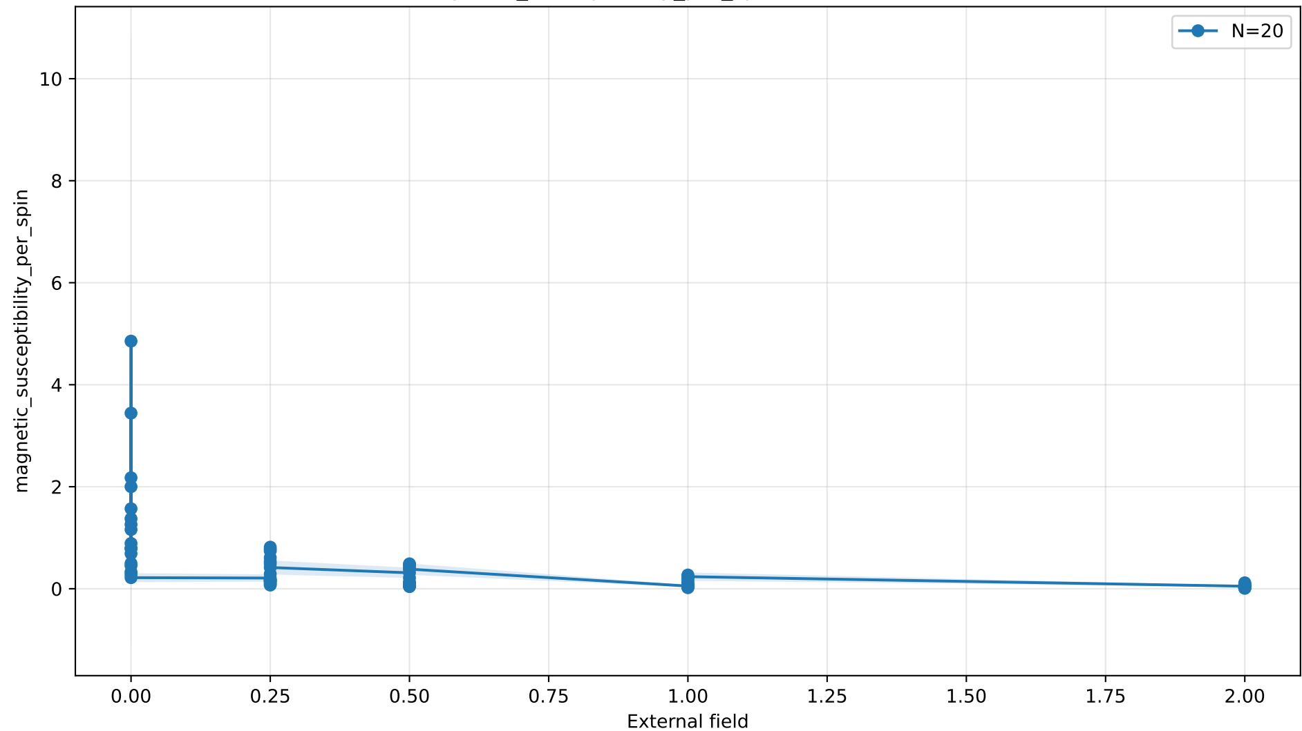
magnetic_susceptibility_per_spin vs external field
