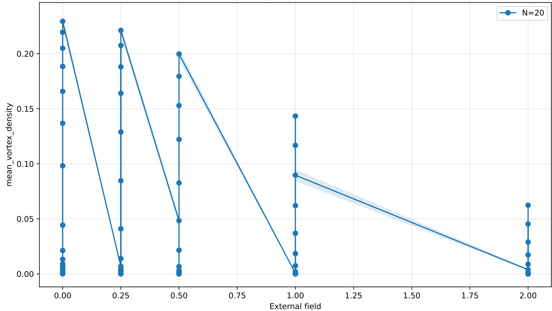
mean_vortex_density vs external field
