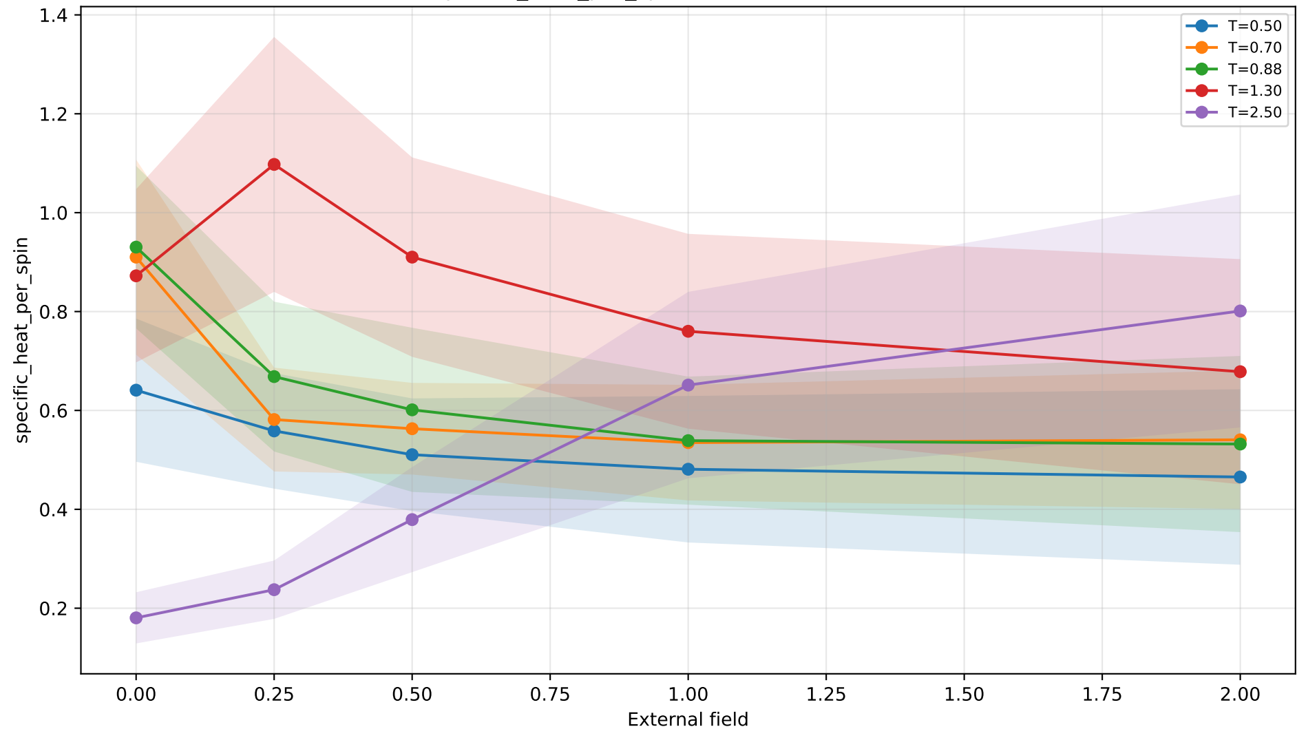
specific_heat_per_spin vs external field, N=20
