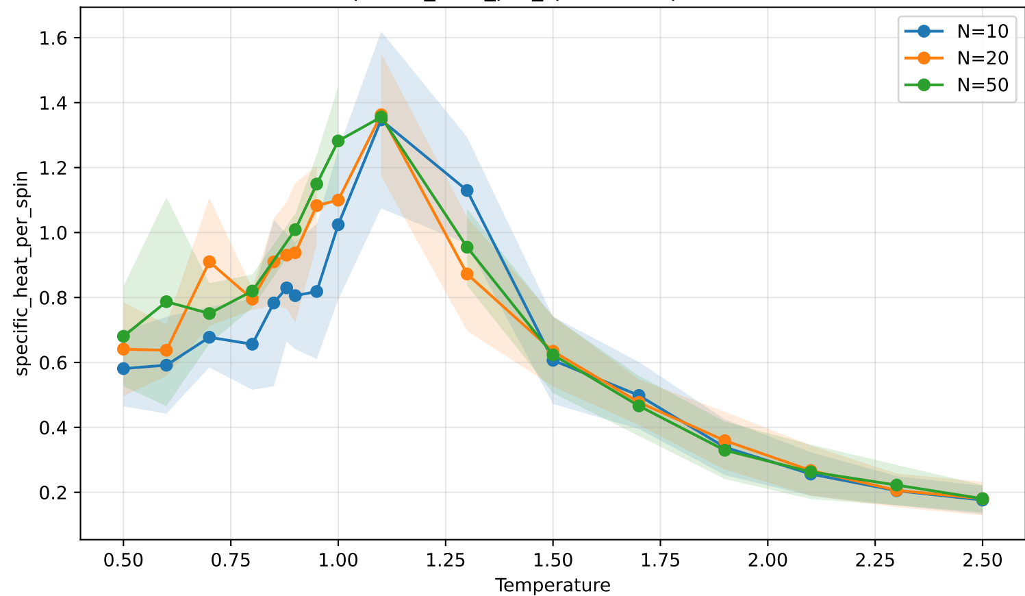
specific_heat_per_spin vs temperature
