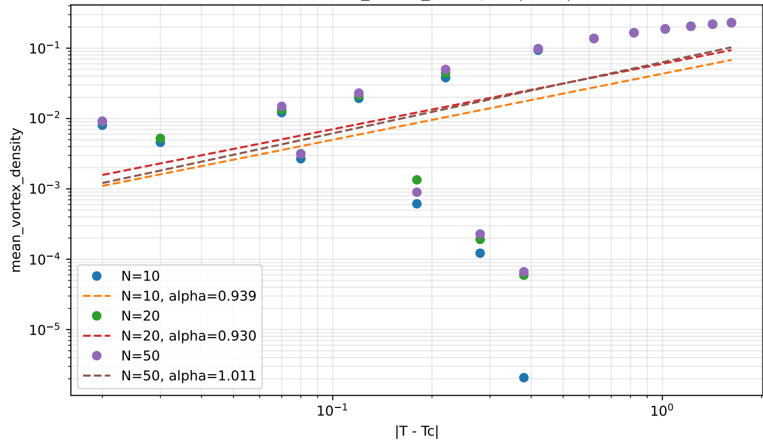
Power-law test: mean_vortex_density vs |T - T_c| , T_c=0.88
