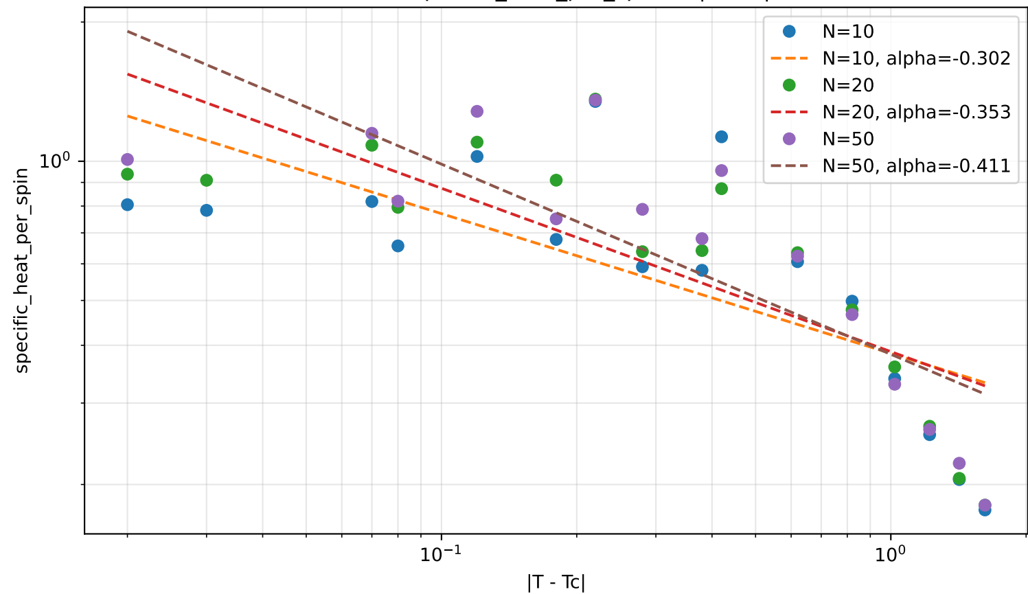
Power-law test: specific_heat_per_spin vs |T - T_c| , T_c=0.88
