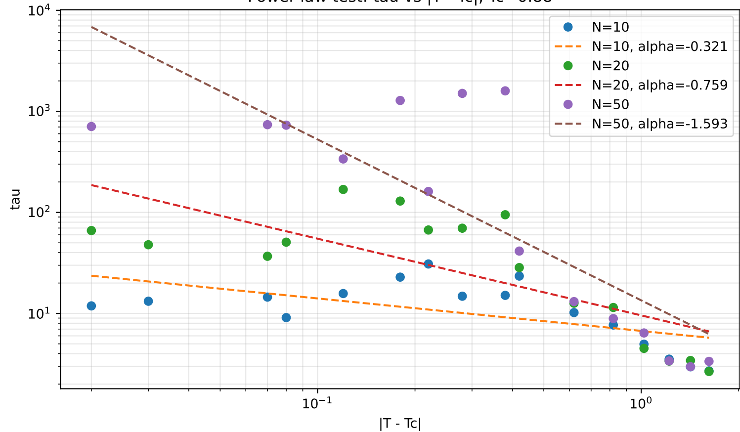
Power-law test: tau vs |T - T_c| , T_c=0.88
