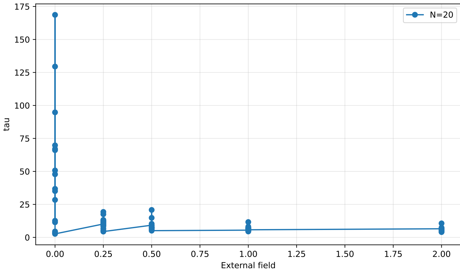
tau vs external field
