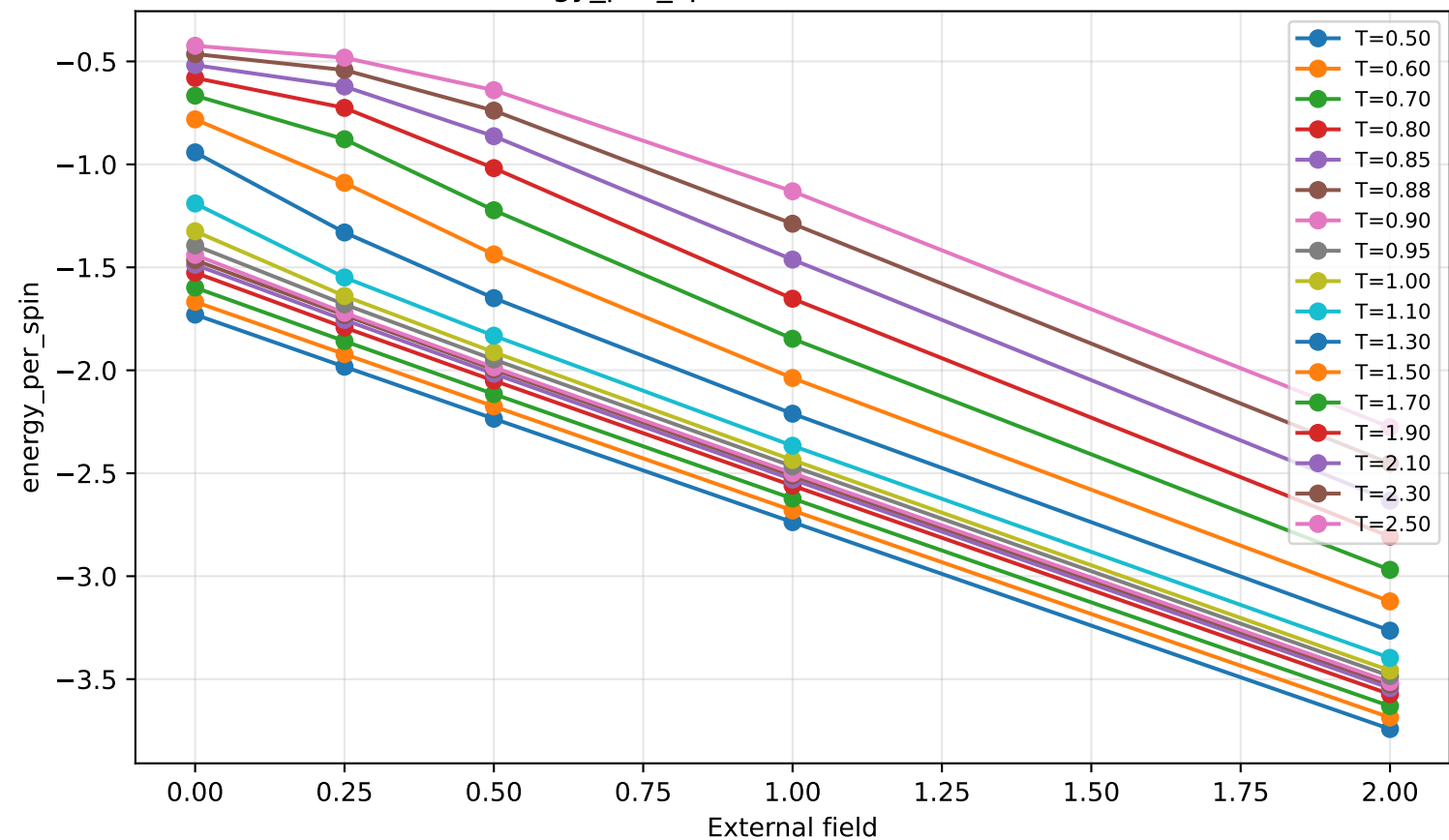
energy_per_spin vs external field, N=20
