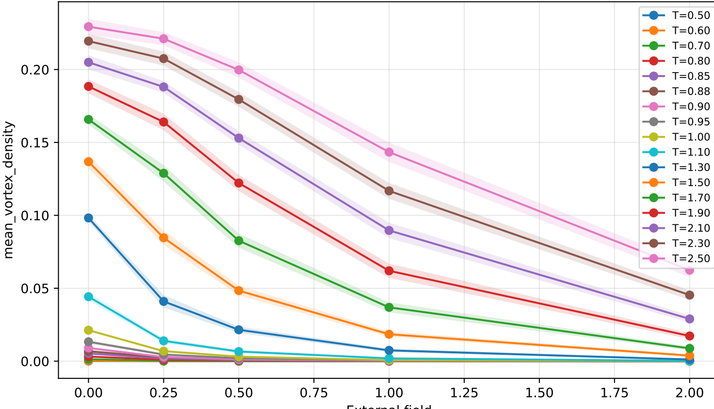
mean vortex density vs external field, N=20
