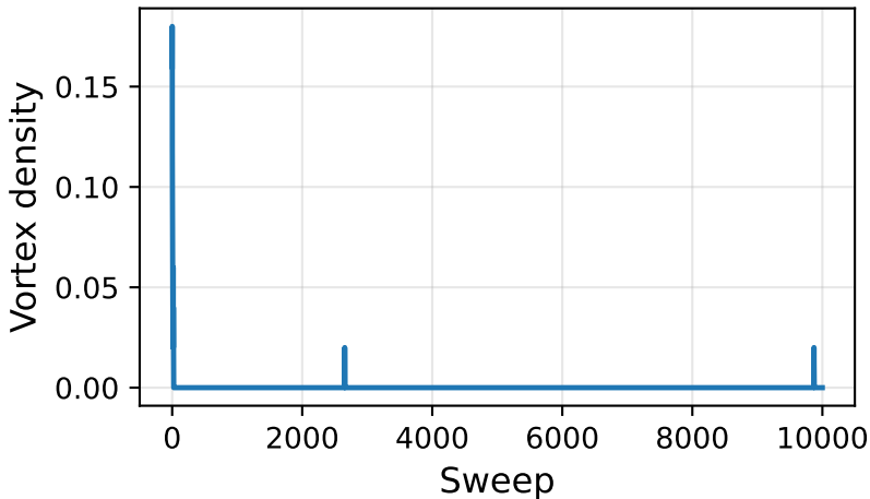
Vortex density vs sweep
