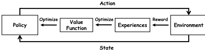
Fig. 3. RL process.
