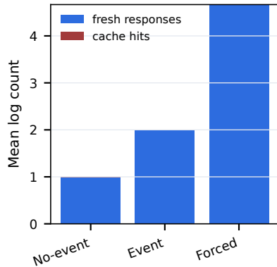
No-cache trace
