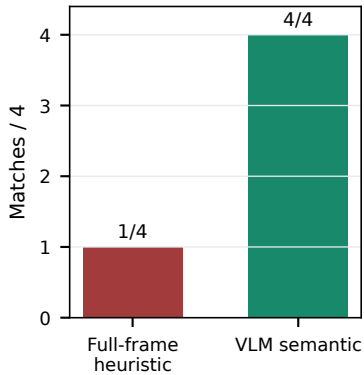
Target-image audit
