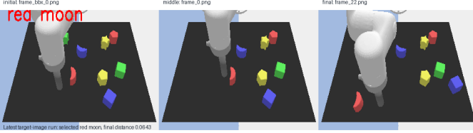
Fig. 5. Representative latest target-image run frames. The quantitative claim is taken from CSV/JSON metrics; the frames provide qualitative evidence that the logged run is a real Language-Table execution rather than a table-only report.
