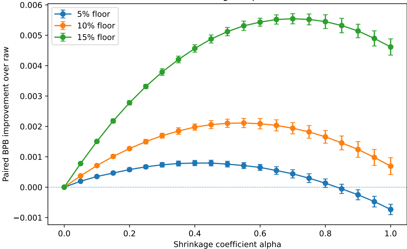
Muon+AdamW: shrinkage response across floors
