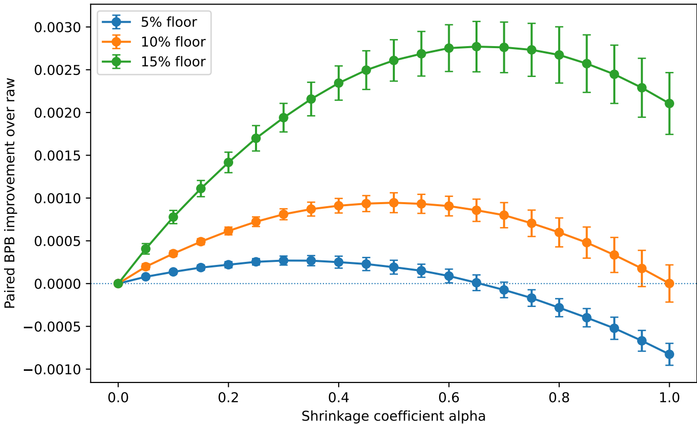
Pure AdamW: shrinkage response across floors
