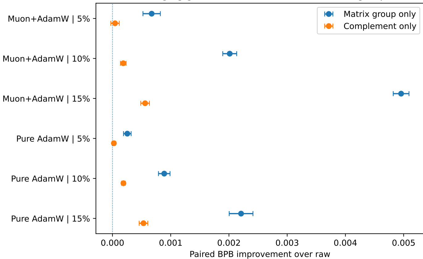
Averaging gain is concentrated in the matrix group
