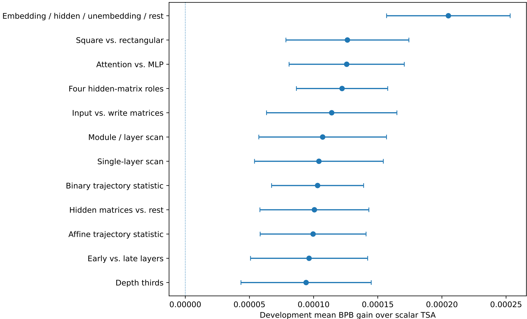
Development search over parameter-group structures
