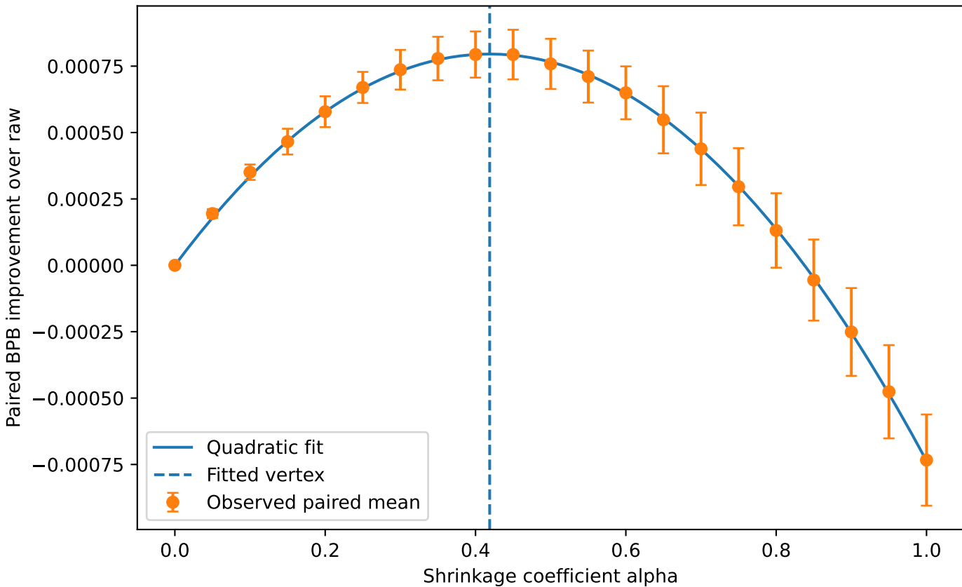
Muon+AdamW | 5% floor | R^2=0.99977
