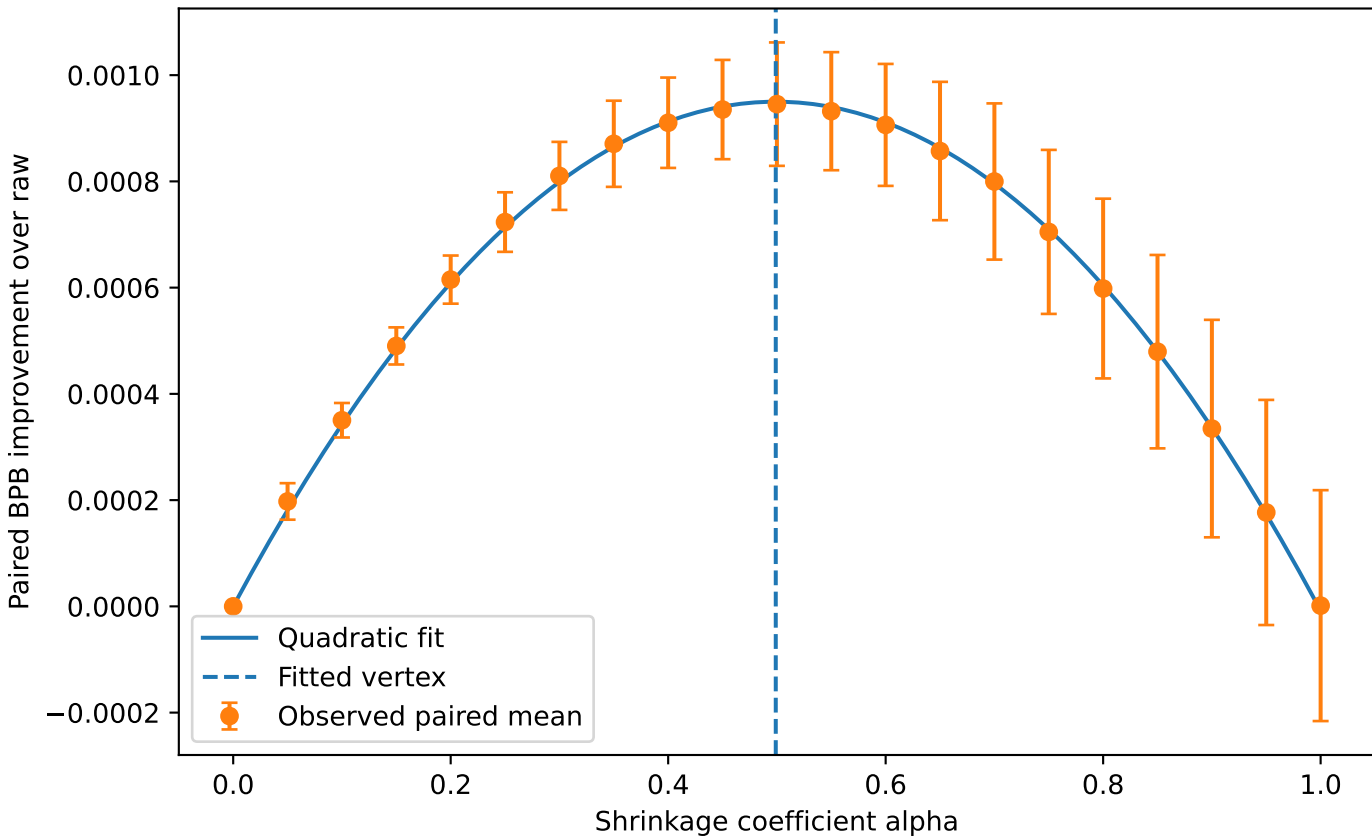
Pure AdamW | 10% floor | R^2=0.99950
