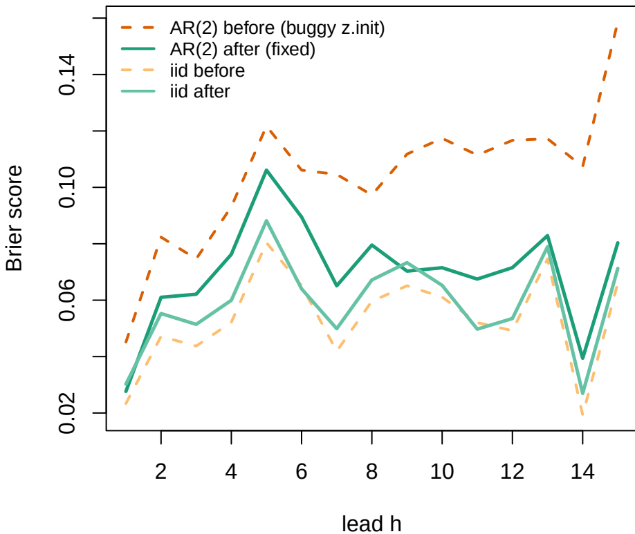
Brier q95, setting 4 (mean over datasets & blocks)
