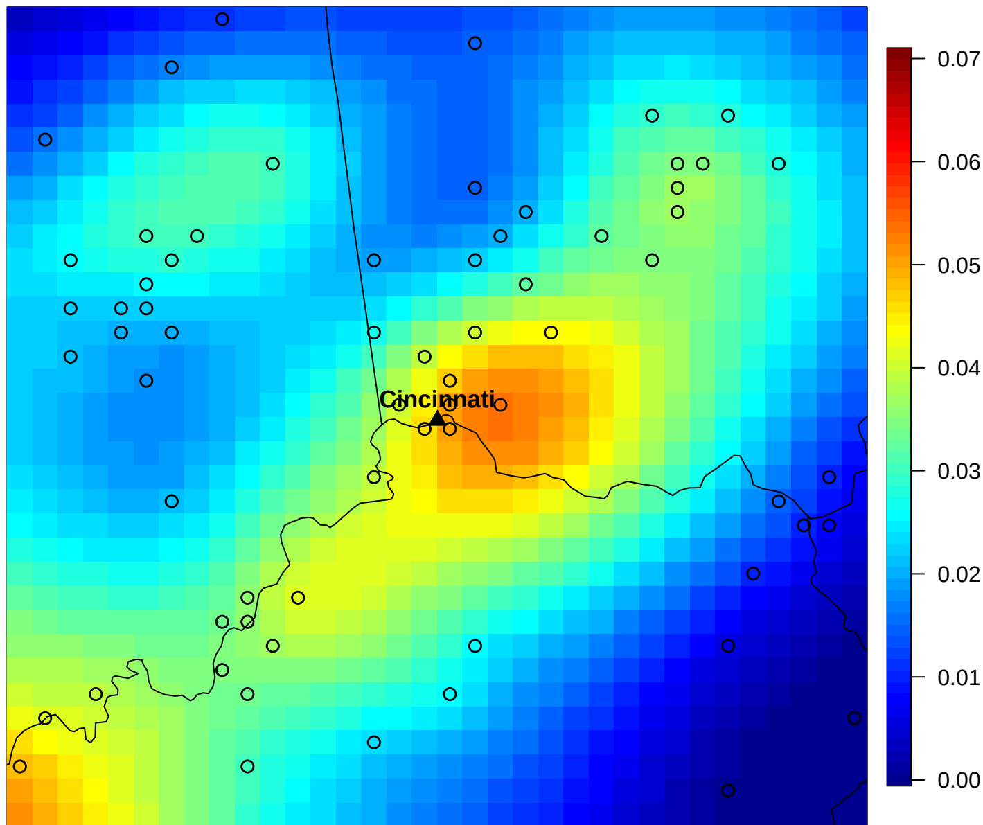
Brier score, exceedance of 75 ppb, setting 204 (MRTS k=10)
