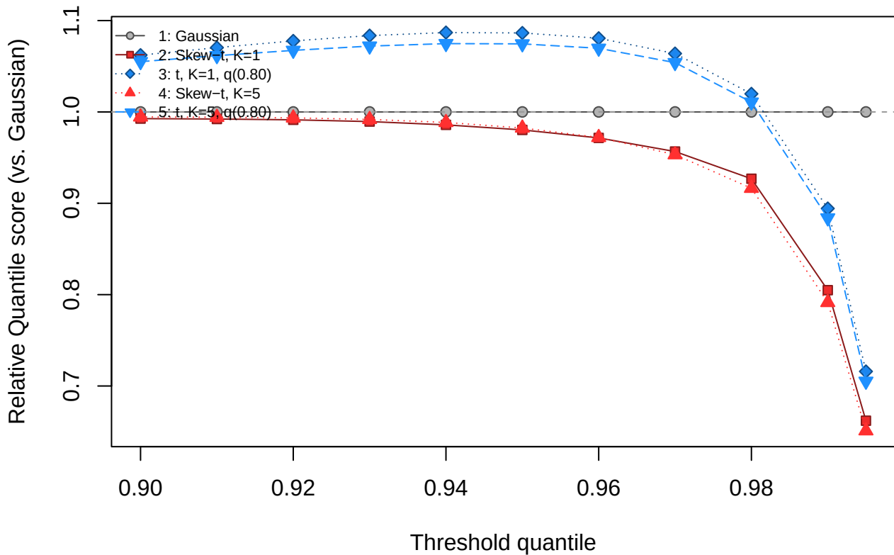
Skew- t ( K=1 , \lambda=3 ), prop_k = 20
