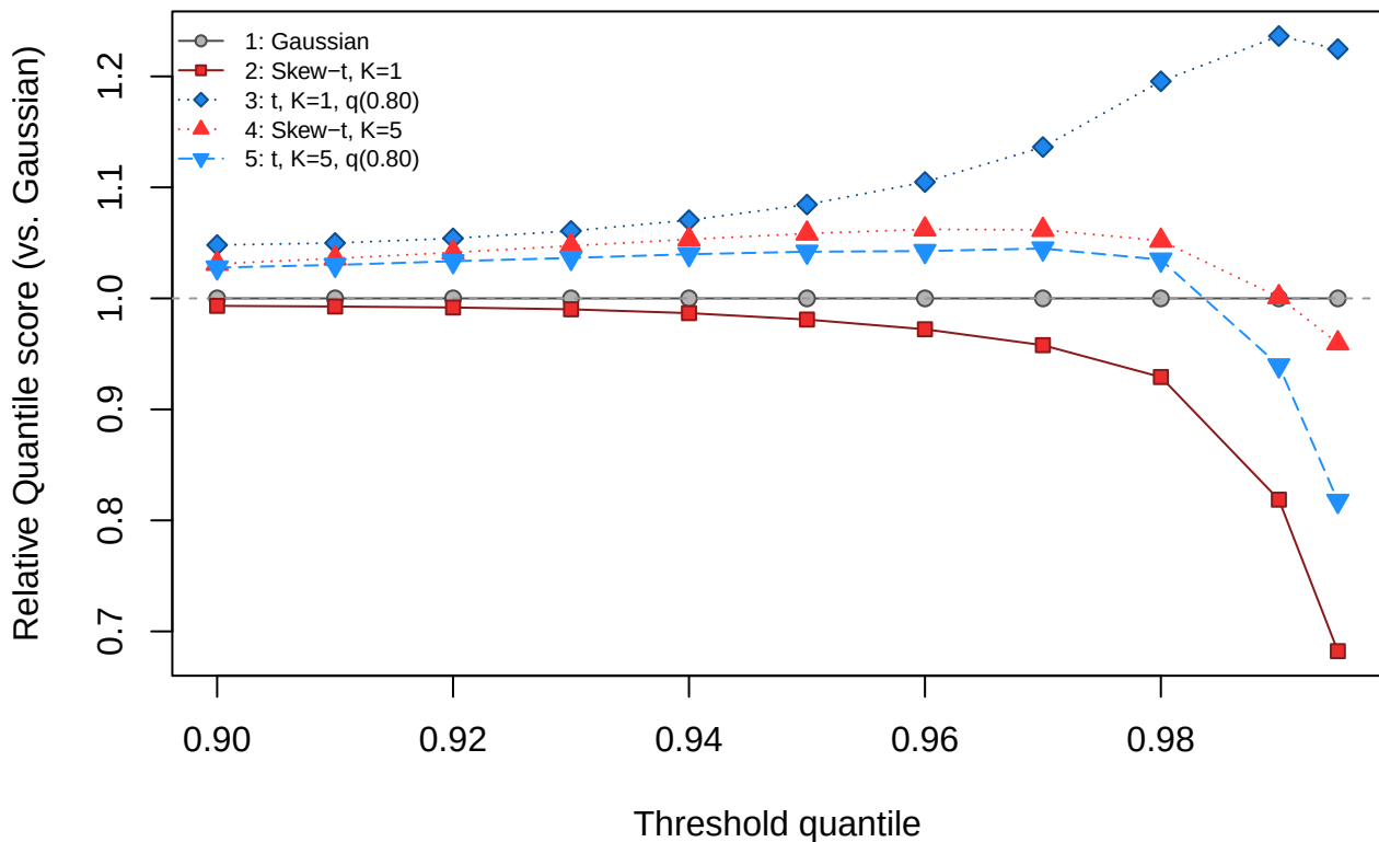
Skew- t ( K=1 , \lambda=3 ), prop_k = 70
