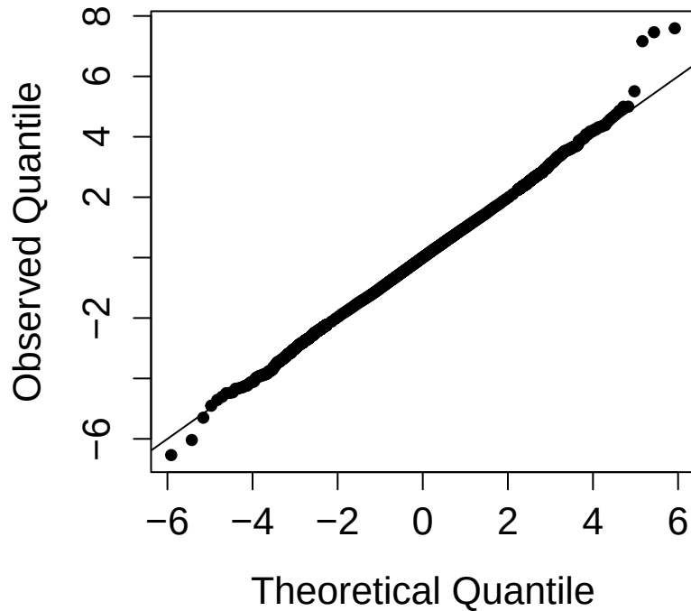
day-standardized alpha=0.02, nu=9.9
