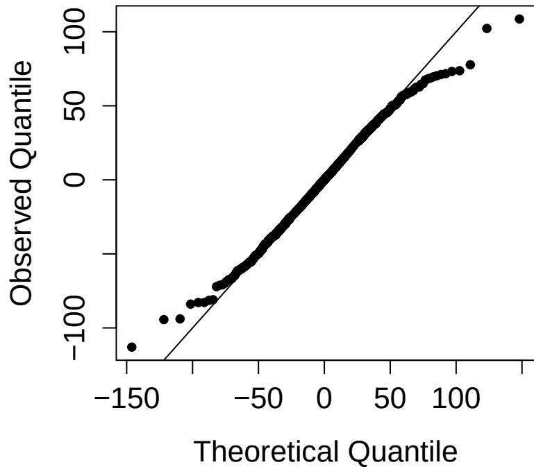
pooled (no day-scaling) alpha=0.02, nu=3.8
