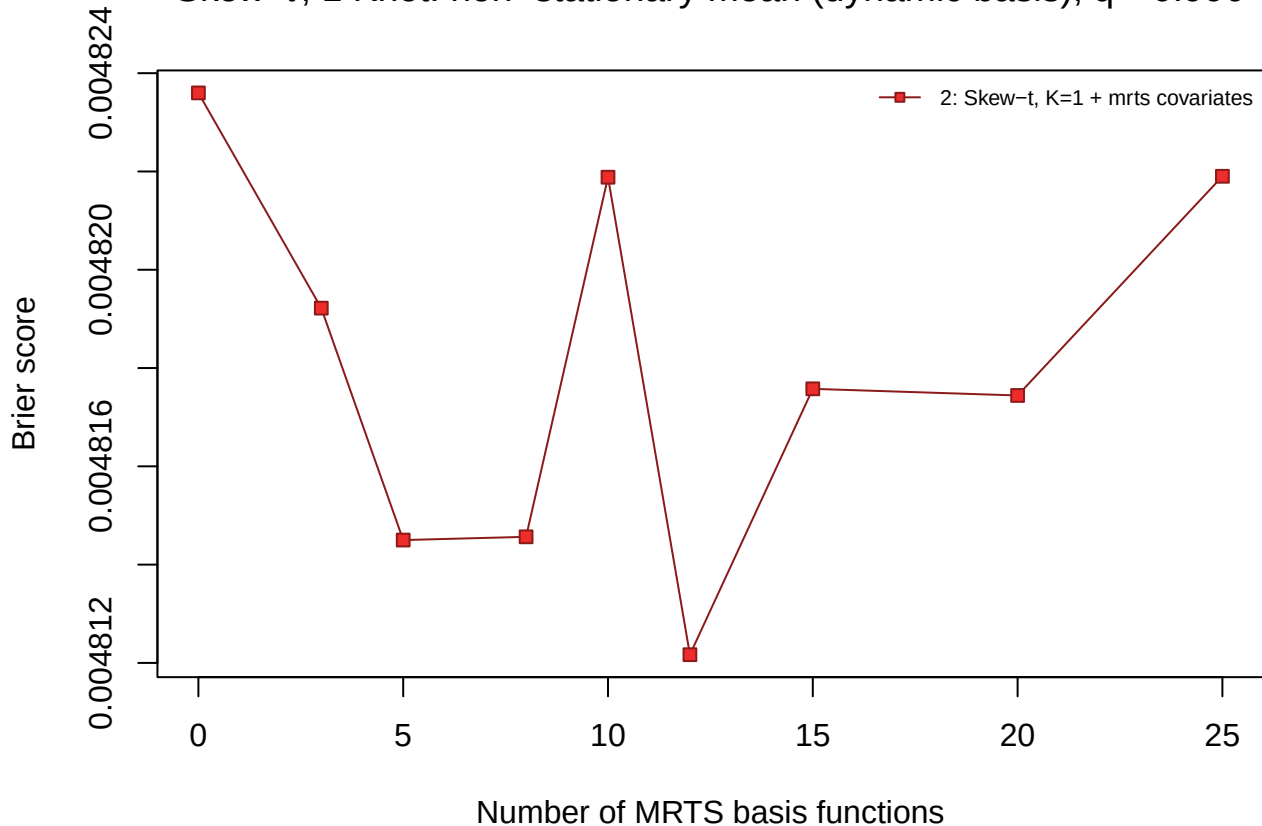
Skew- t , 1 Knot: non-stationary mean (dynamic basis), q = 0.990
