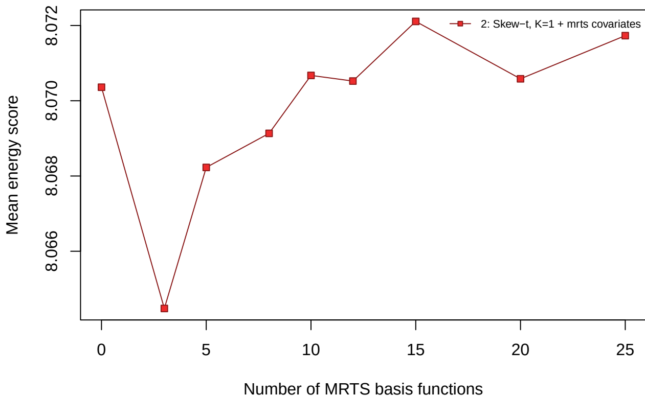
Skew- t , 1 Knot: non-stationary mean (dynamic basis)
