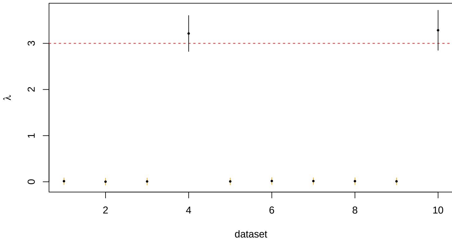
95% CI for lambda – method 4, mrts_k = 8
