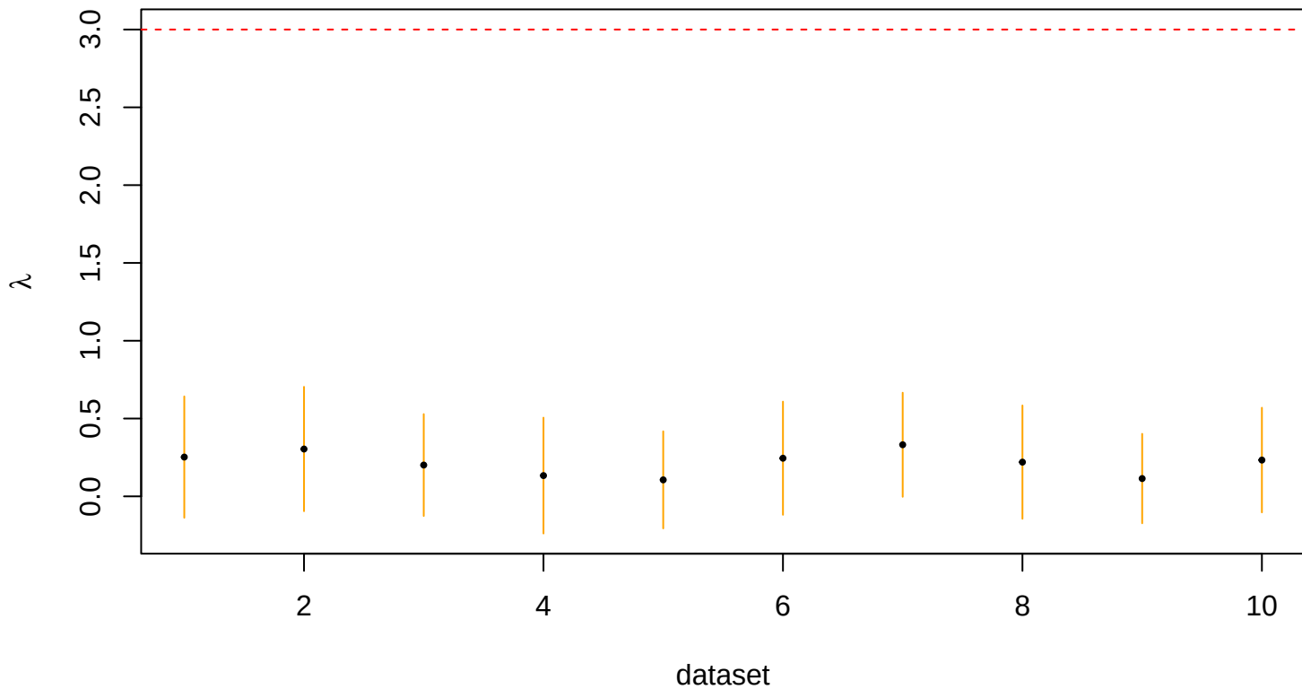
95% CI for lambda – method 2, mrts_k = 8
