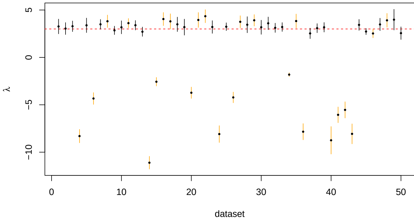
95% CI for lambda — method 2, prop_k = 30
