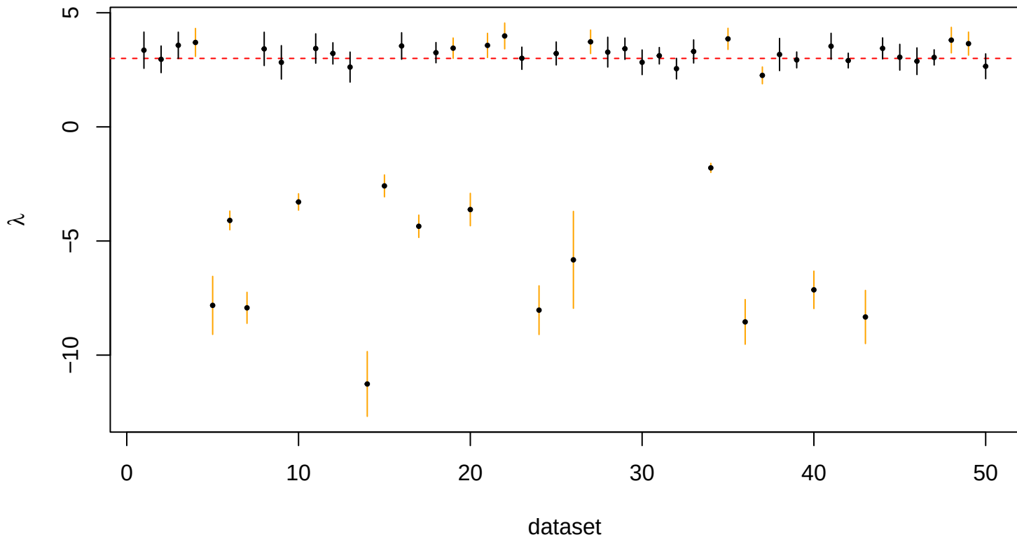
95% CI for lambda — method 2, prop_k = 50
