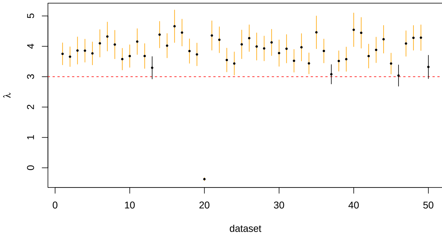
95% CI for lambda — method 4, prop_k = 10
