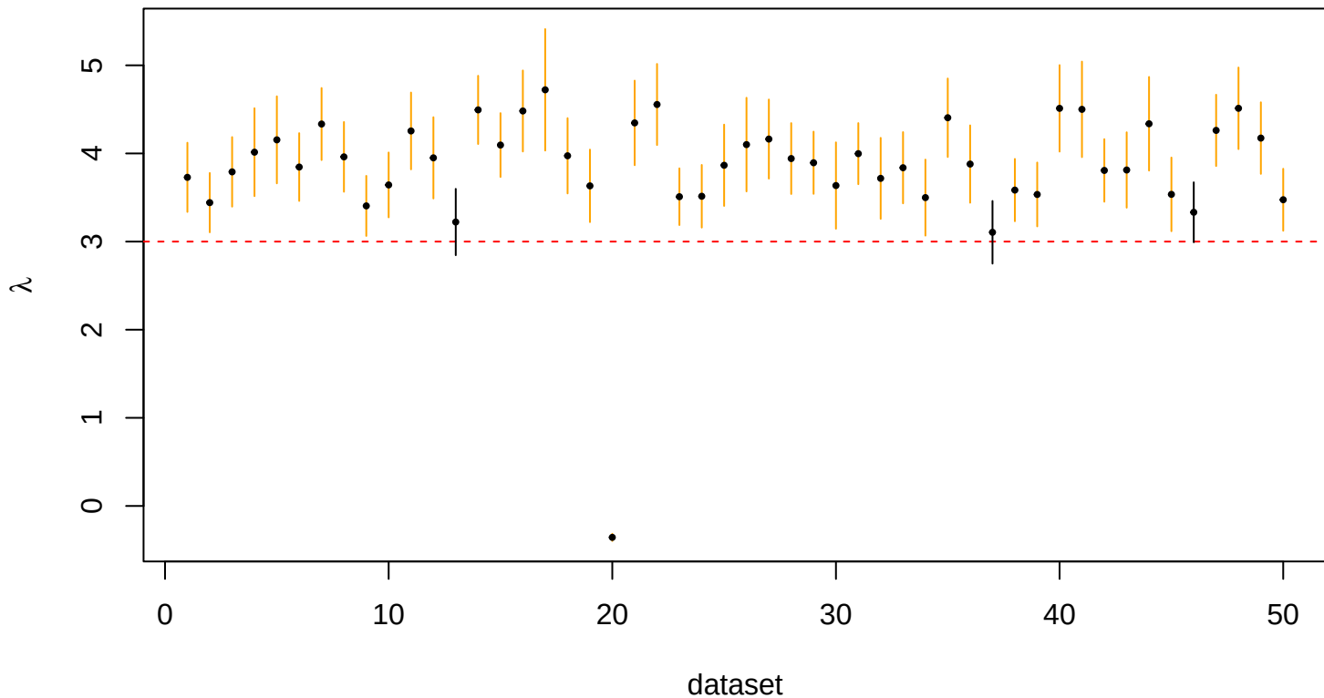
95% CI for lambda — method 4, prop_k = 20
