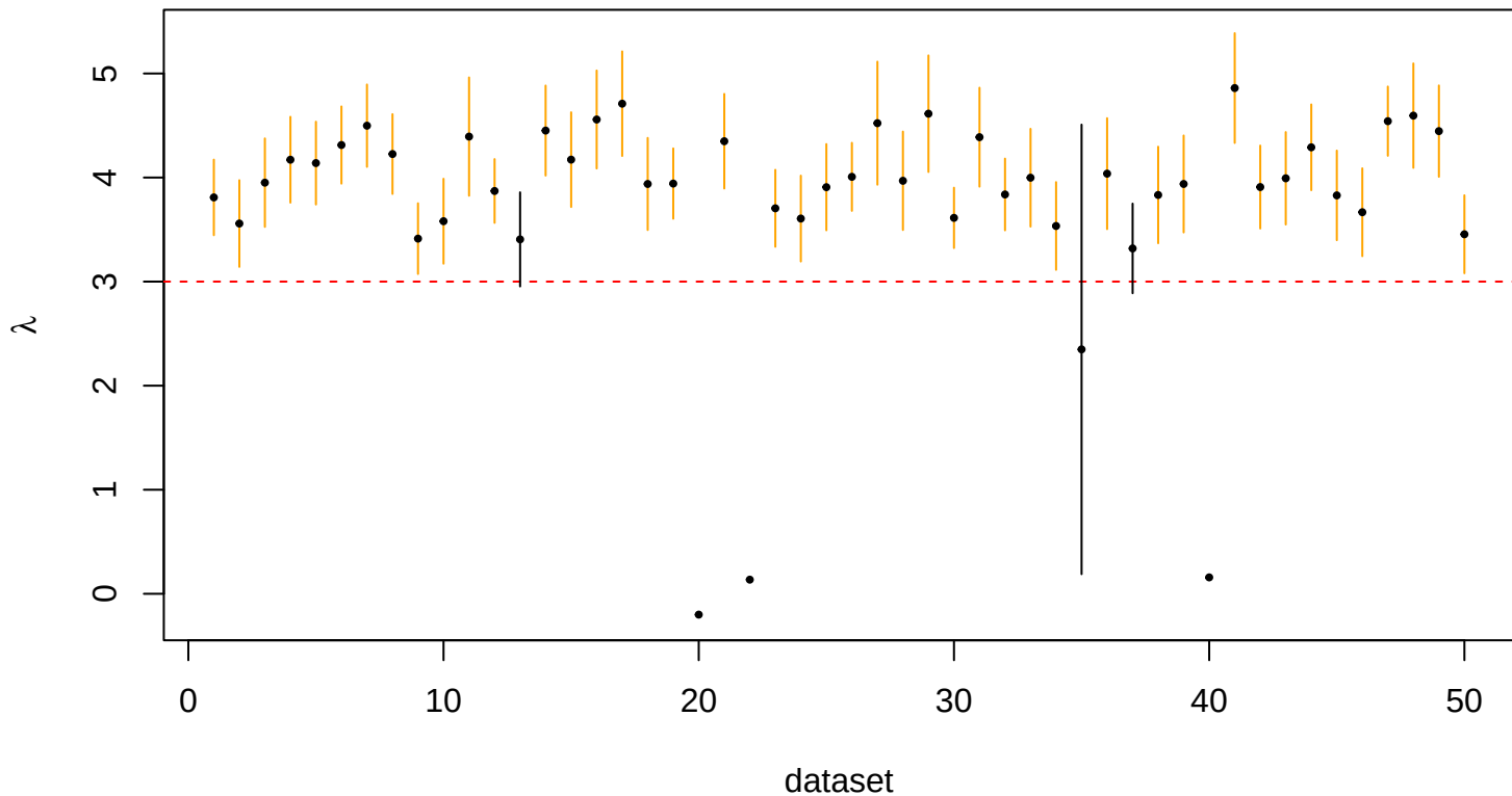
95% CI for lambda — method 4, prop_k = 40
