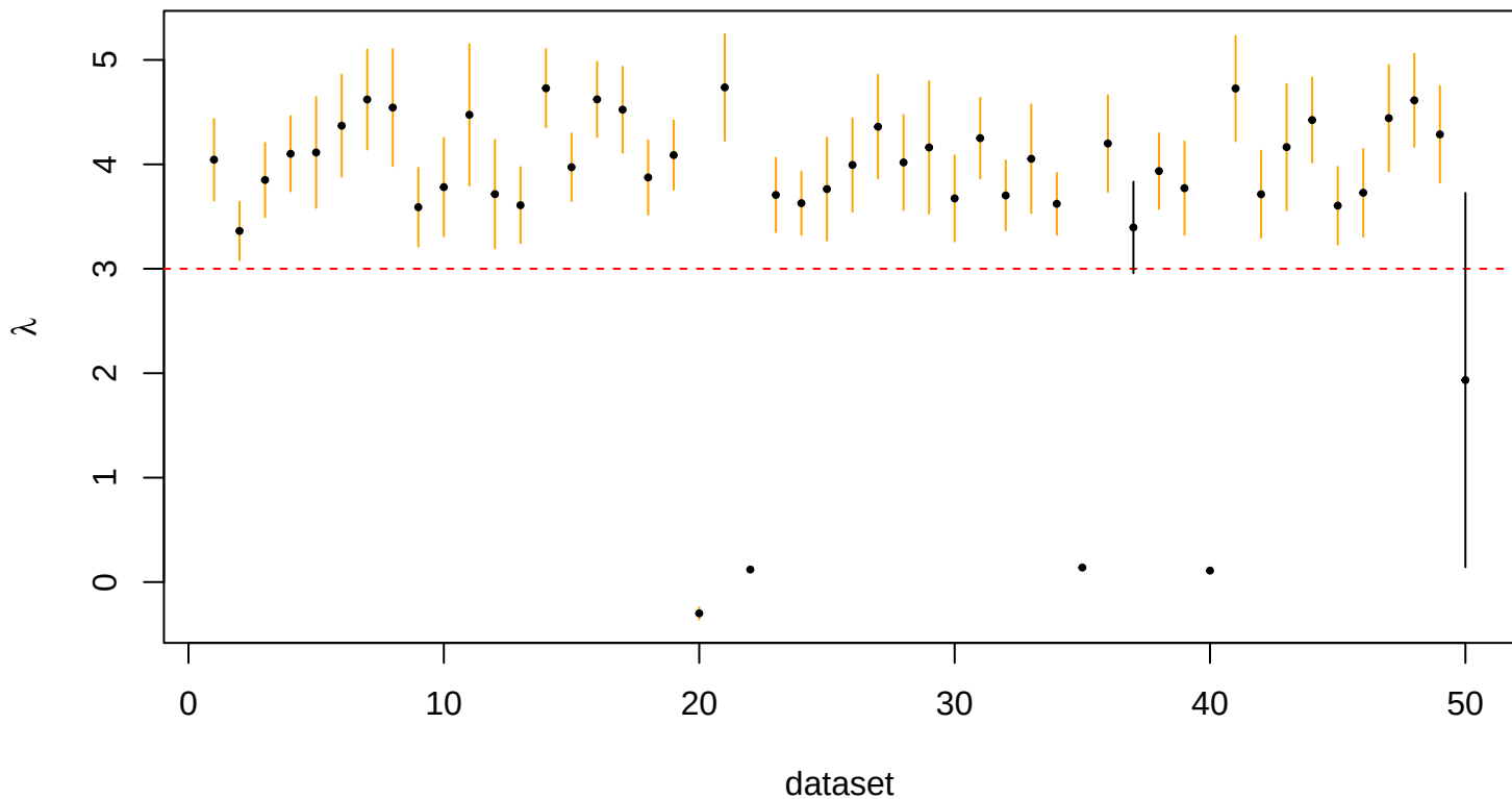
95% CI for lambda — method 4, prop_k = 50
