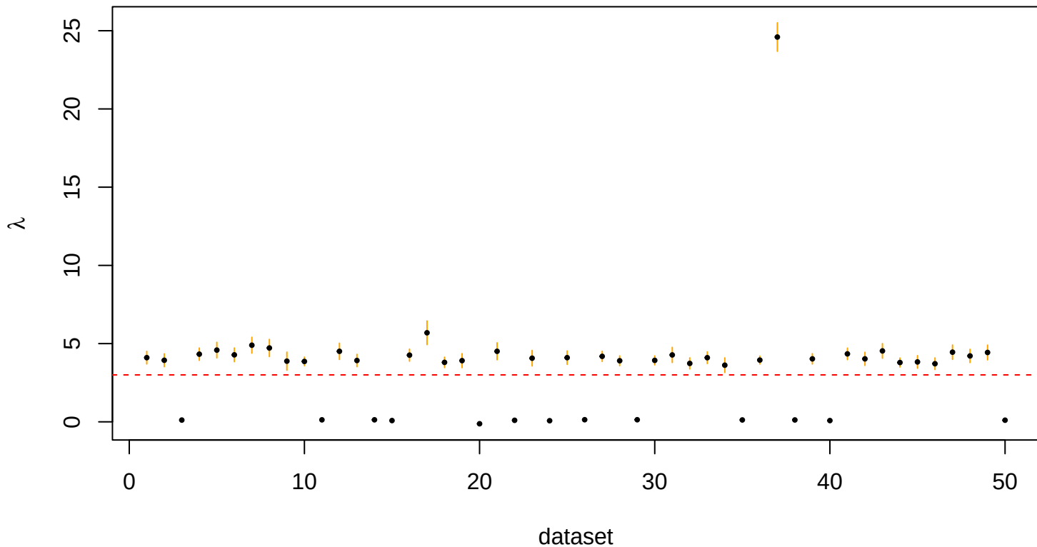
95% CI for lambda — method 4, prop_k = 70
