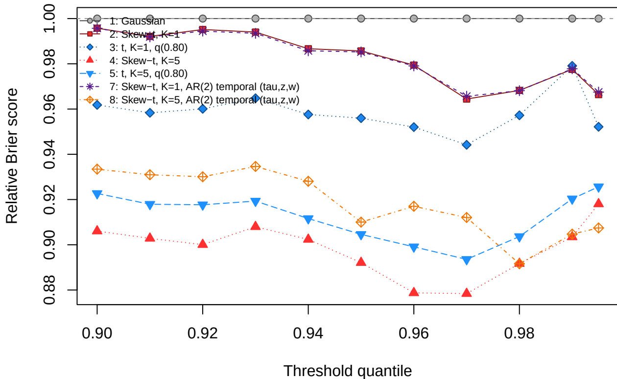
Skew- t ( K=5 , \lambda=3 ), AR(2): \phi_1=0.8 , \phi_2=-0.35
