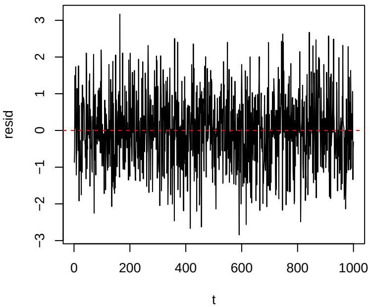
Residuals – manual recursion
