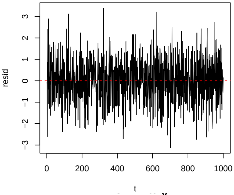
Residuals - filter()
