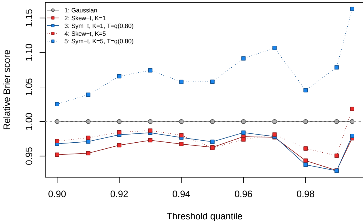
Skew- t ( K=1 , \lambda=3 ), geometric anisotropy ( \theta=\pi/4 , r=0.5 )
