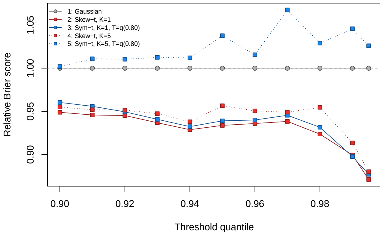
Skew- t ( K=1 , \lambda=3 ), geometric anisotropy ( \theta=\pi/6 , r=0.25 )
