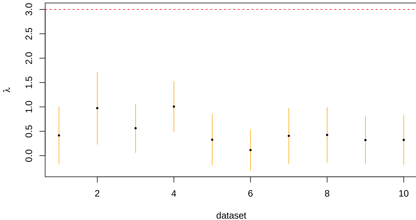
95% CI for lambda – method 2, mrts_k = 20
