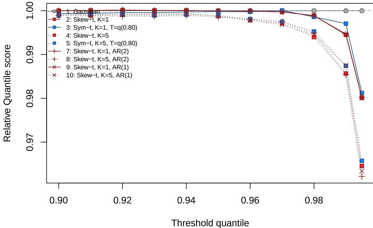
Skew- t ( K=5 , \lambda=3 ), AR(2): \phi_1=0.12 , \phi_2=-0.05
