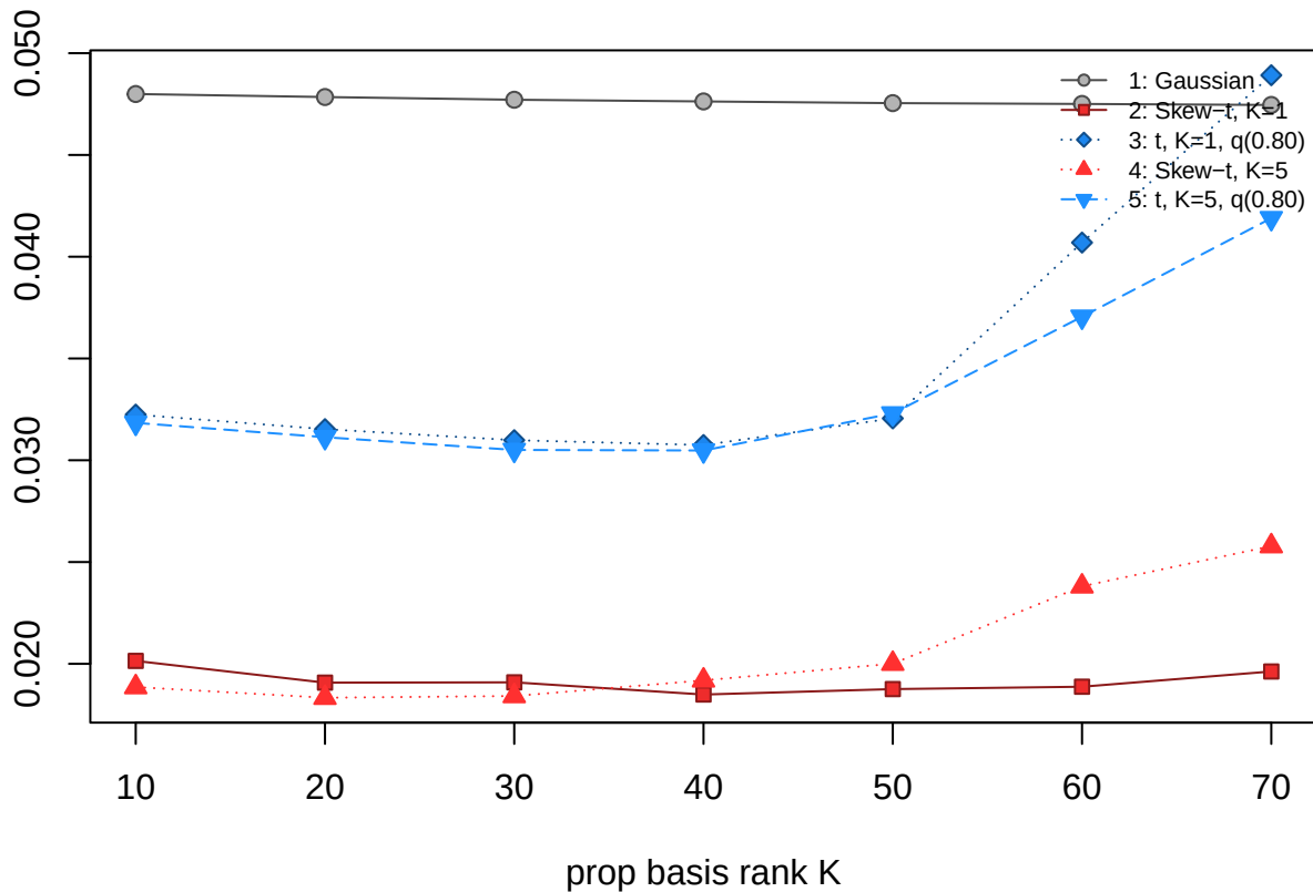
Skew- t ( K=1, \lambda=3 )
