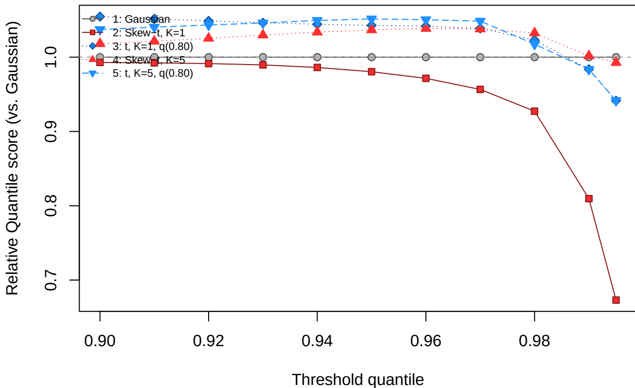
Skew- t ( K=1 , \lambda=3 ), prop_k = 60
