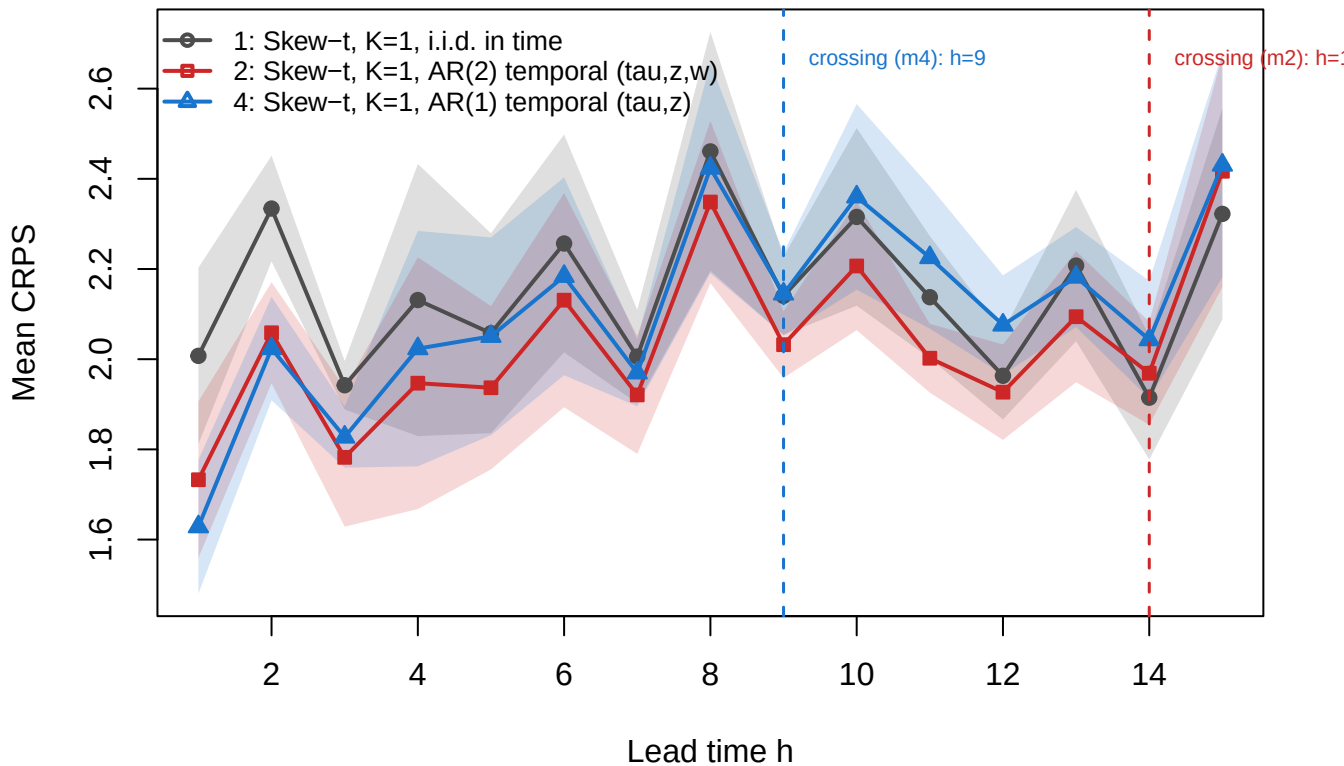
Lead-time curve – Skew- t ( K=1 , \lambda=3 ), ARFIMA d=0.45 ( H=0.95 )
